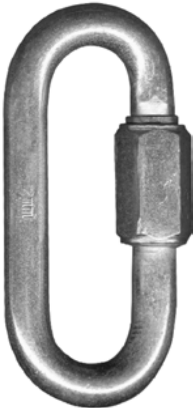
QL57 1/2" steel wire, zinc 4 3/16" length 9/16" gate opening
