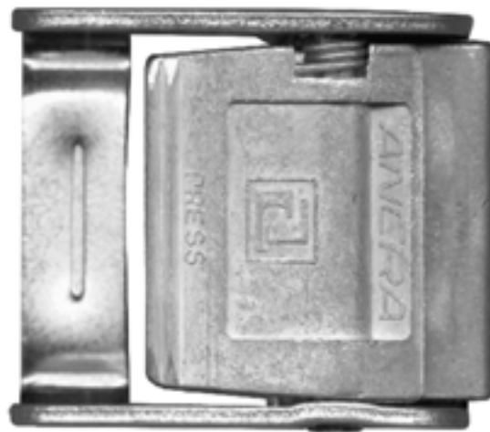
CAM/200-3000 2" steel, zinc chromate 3,000 lb
