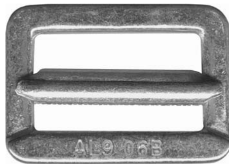
AL9 knurled adjuster bar 1 3/4" x 1" forged steel, zinc plated 5,000 lb Commercial version of PS22040 Use RH9 for certified PS22040 version.
