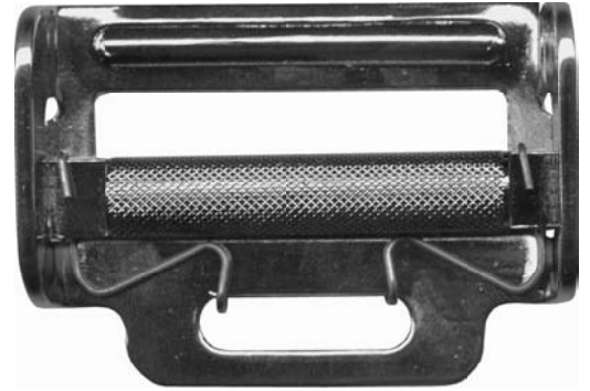
AL14-S Roller Adjuster with Spring Tensioner 2" slot alloy steel, chrome plated 1,000 lb
