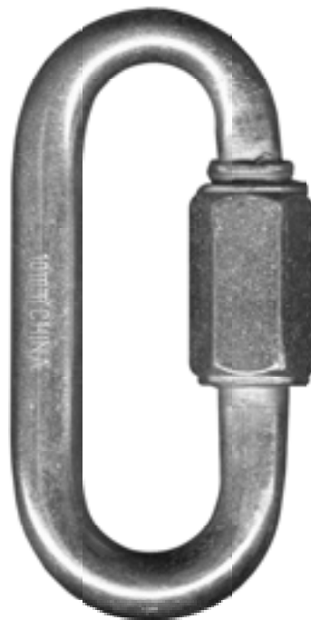
QL56 13/32" steel wire, zinc 3 1/2" length 1/2" gate opening
