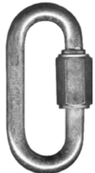
QL54 5/16" steel wire, zinc 3" length 3/8" gate opening Use QL68 for Stainless Steel
