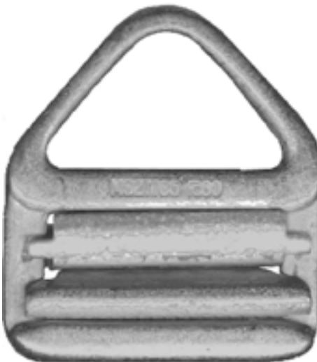
RH20 Adjustable with Tension Spring 1 3/4" slot forged steel, cadmium plated 2,500 lb. proof load Certifies to PS27765 SPECIAL ORDER
