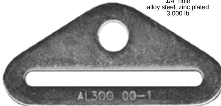
AL300 Bolt-In End Fitting 3" x 1/4" slot, 1/2" hole alloy steel, zinc plated 5,000 lb.
