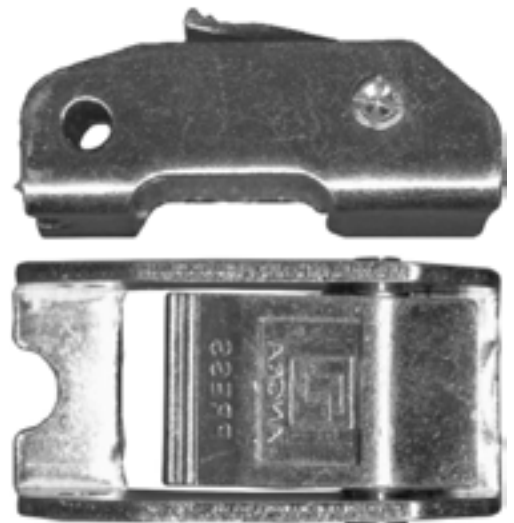
CAM/100-1500 1" steel, cadmium 1,500 lb
