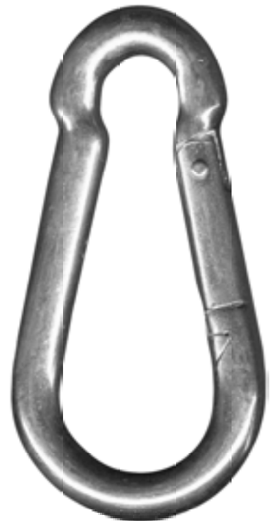
SPC60 13/32" steel wire, zinc 3 7/8" length 9/16" gate opening Use SP74 for Stainless Steel
