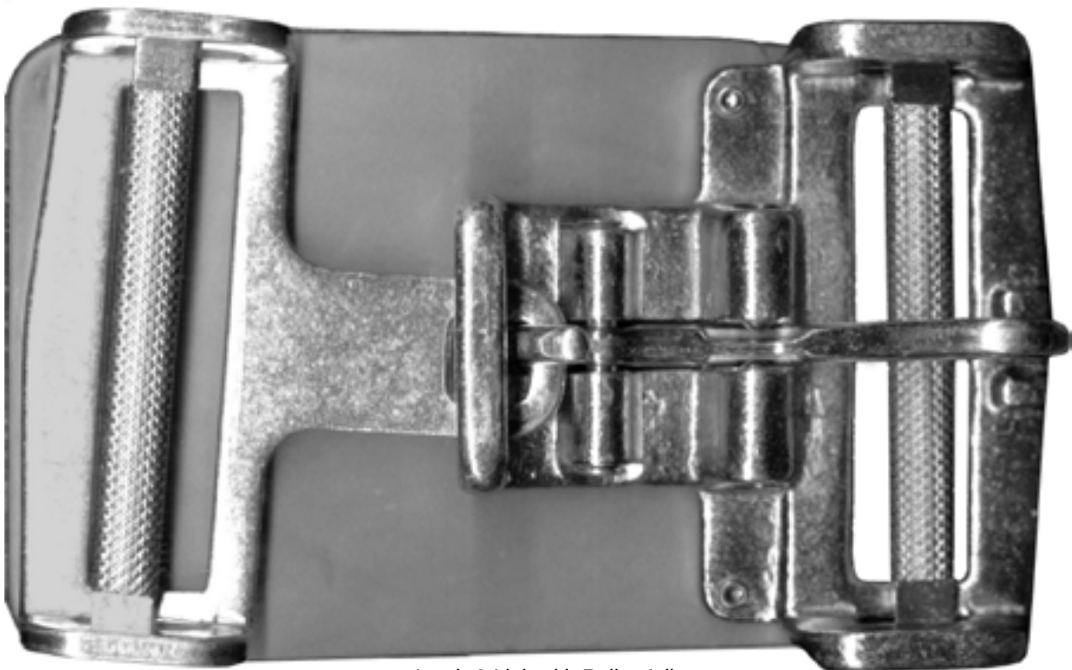
Latch & Link with Roller Adjusters with leather pad RH7116 3" forged steel, zinc plated 3,000 lb
