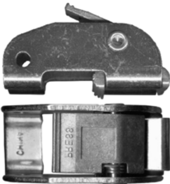
CAM/100-1800 1" steel, cadmium 1,800 lb
