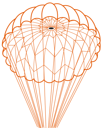
PARACHUTE/88-NASA 88' Apollo Recovery Chute Slotted canopy only Orange & White
