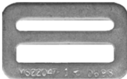
RH6 1 3/4" slots alloy steel, cadmium plated 1,000 lb. proof load Certifies to PS22047 Also available in black phosphate
