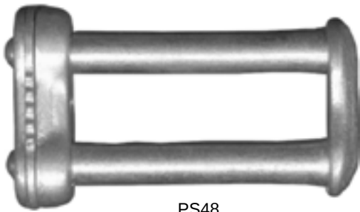
PS48 Separable Link 1 3/4" forged steel, cadmium plated Surplus version of MS70118
