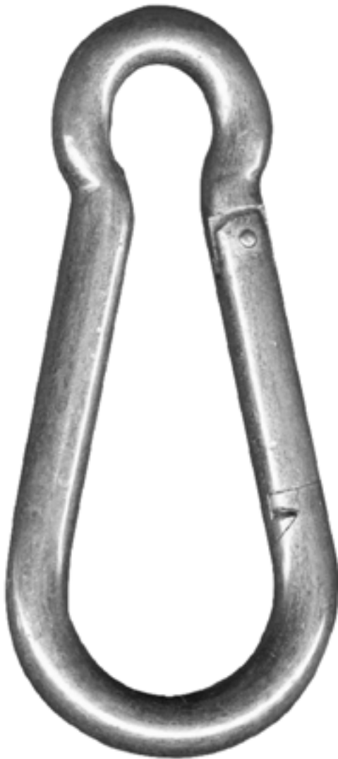
SP58 1/2" steel wire, zinc 5 1/2" length 3/4" gate opening
